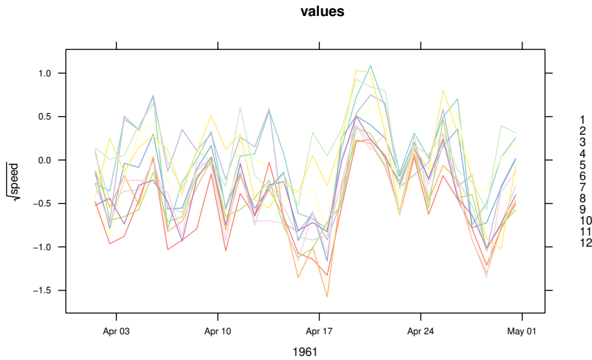
Figure 7: Time series plot of daily wind speed at 12 stations, used for interpolation in Figure 4.
